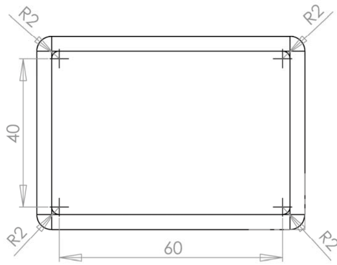
HeinrichsWeikamp OSTC Protection Cover Layout
